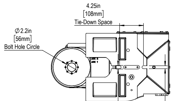
BOTTOM HOLE DIMENSIONS
