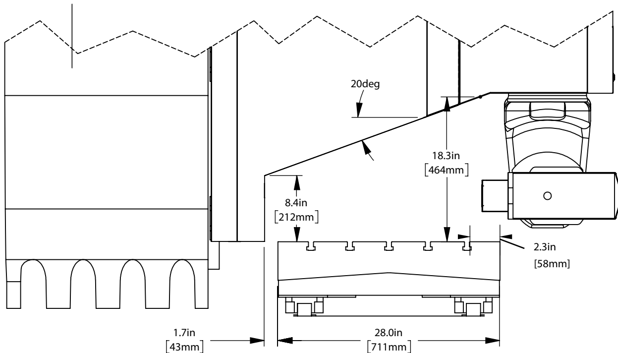
Potential interference at maximum Z travel with Z axis casting
